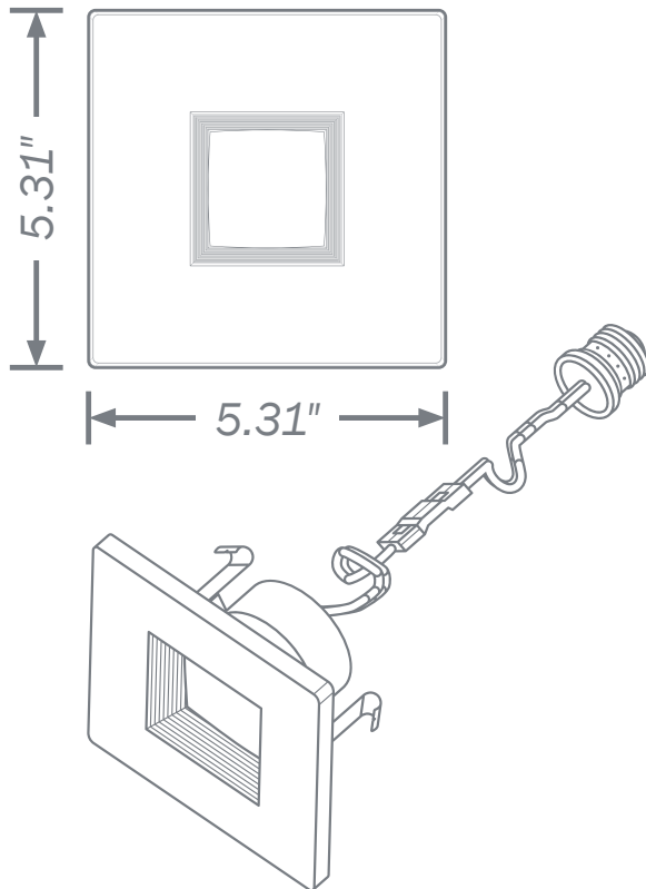
Square baffle snap-in dimensions
